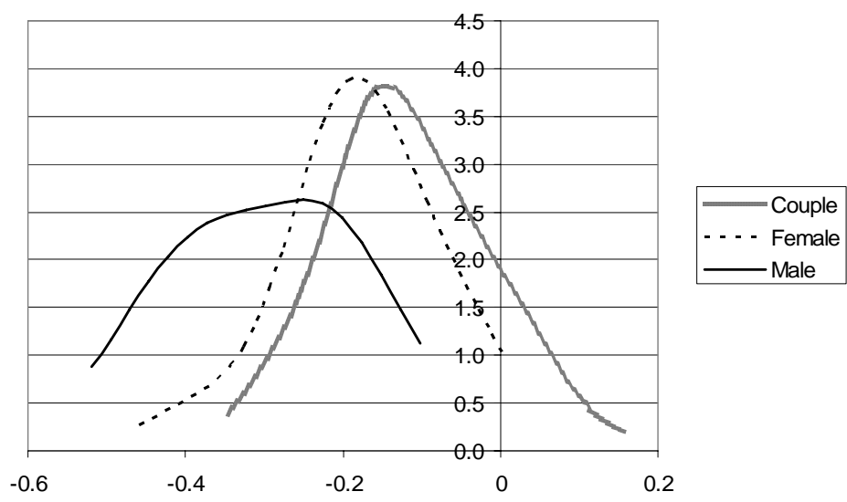
Figure 5. Fitted Conditional Distributions of Marginal values (Price, Pesticide and Fat)
